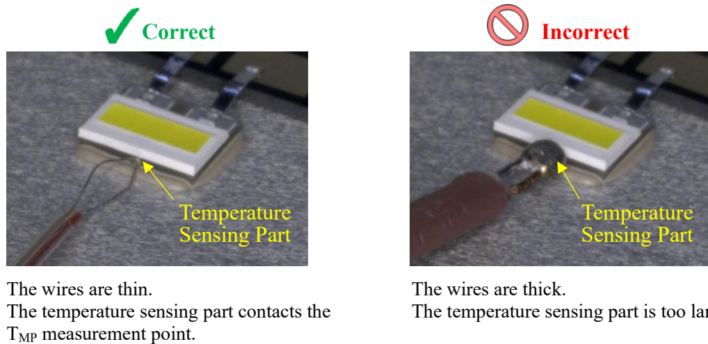
Figure 2. Examples of Correct/Incorrect Thermocouples (Before adhesive is applied)
